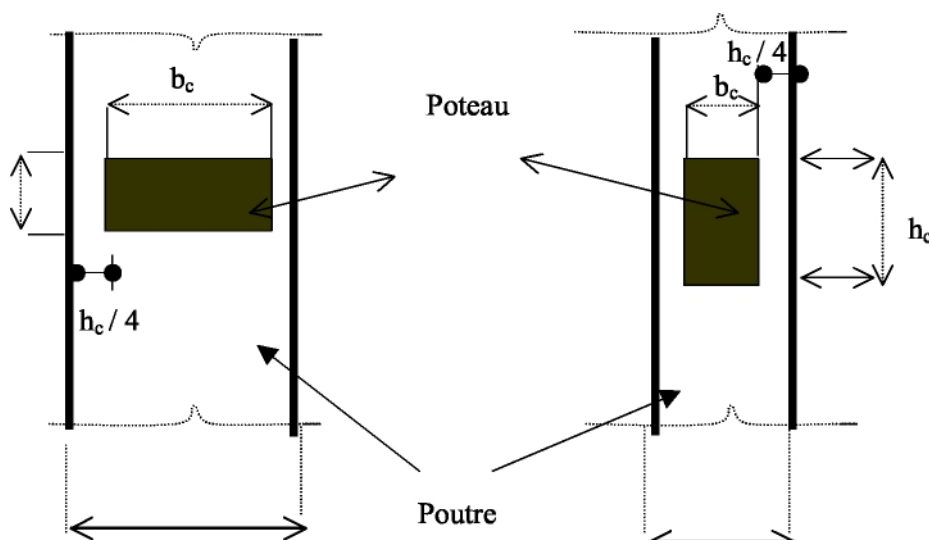
Figure 7.2 : Position poteau-poutre
