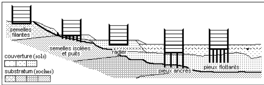
Figure 4.3.2.4 – Types de fondations
